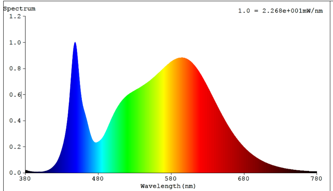
Spectral Distribution
